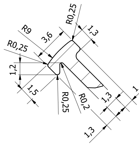
B ( 5/1 ) DETAIL
