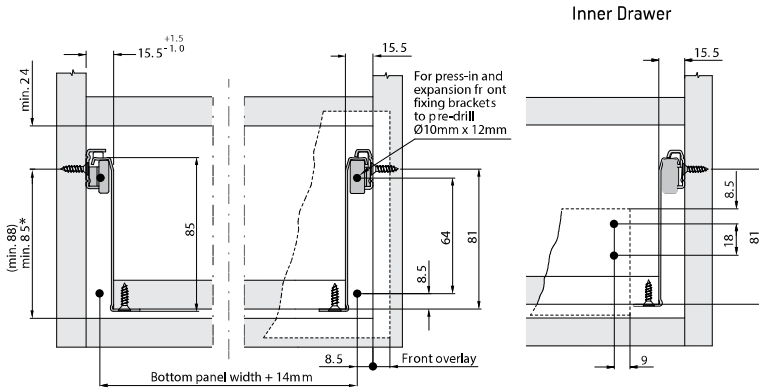
( ) Inner Drawer * Add 8mm when used with 201.000 Drawer Front Locking Piece.
