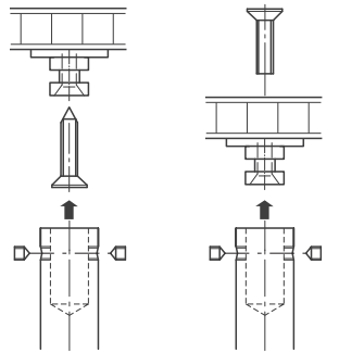
Montage-Variante Spanplatten- schraube Hospa
